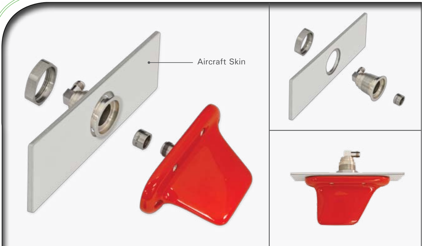
Blind Mate Antenna Connector
